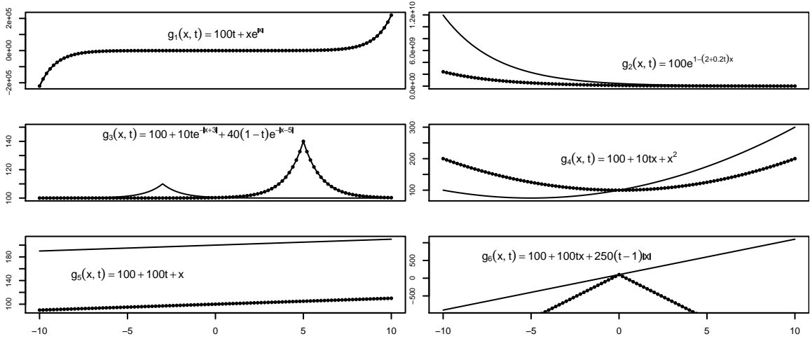
Figure 3: Graphs of x horizontally by g_k(x, t) vertically, for lines k = 1, \dots, 6 . In each, the functions generating the treated t = 1 (solid lines) and control t = 0 (dotted lines) groups appear.
