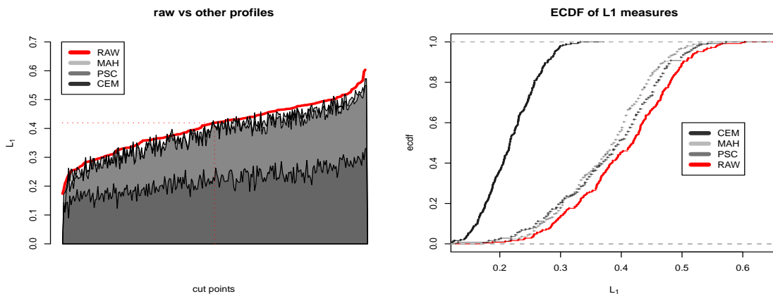
Figure 2: The \mathcal{L}_1 -profile of the raw (“RAW”) data (red line) compared to propensity score (“PSC”), Mahalanobis (“MAHF”) and Coarsened Exact Matching (“CEM”) matched data. MAHF and PSC overlaps in the left panel. The left panel plots the L_1 profile by different bin choices sorted by L_1 for the raw data; the right panel plots the empirical cumulative distribution functions of the same set of \mathcal{L}_1 values.
