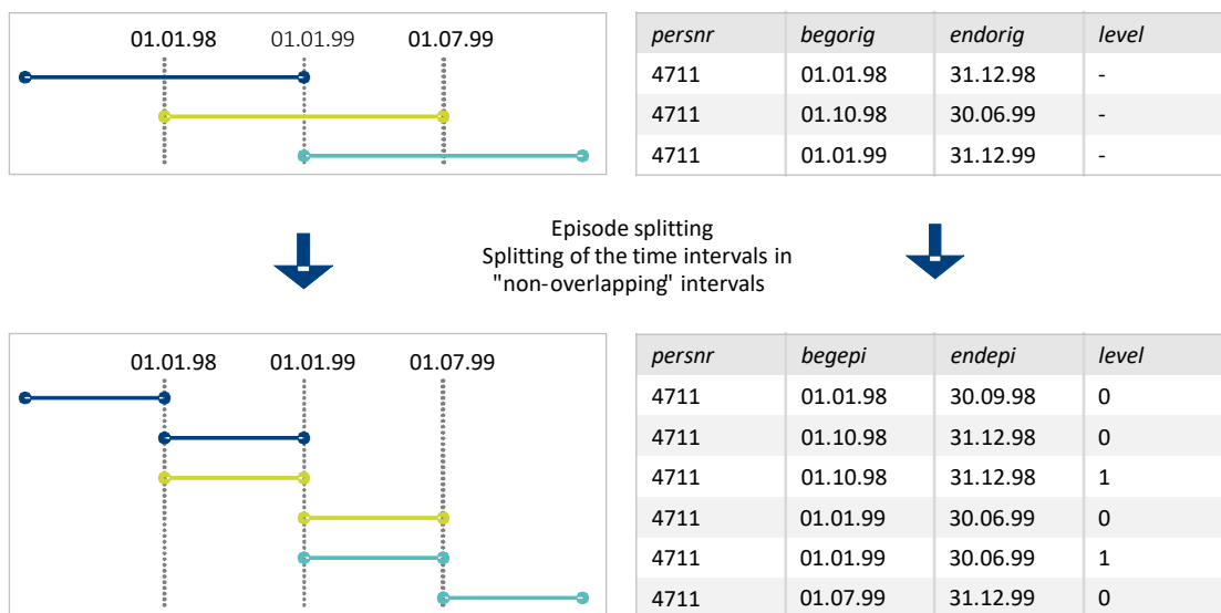
Figure 3: Episode splitting
