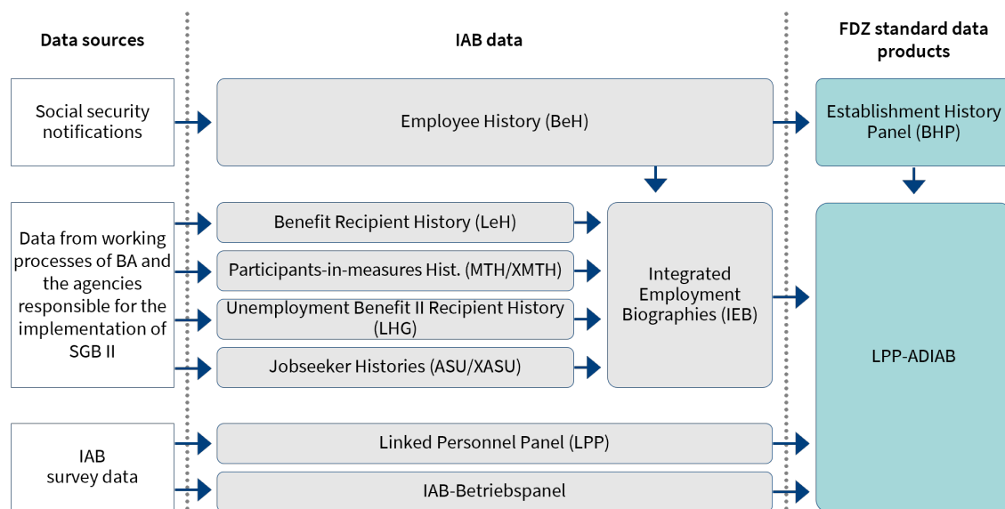
Figure 2: Data sources of the LPP-ADIAB 7524
