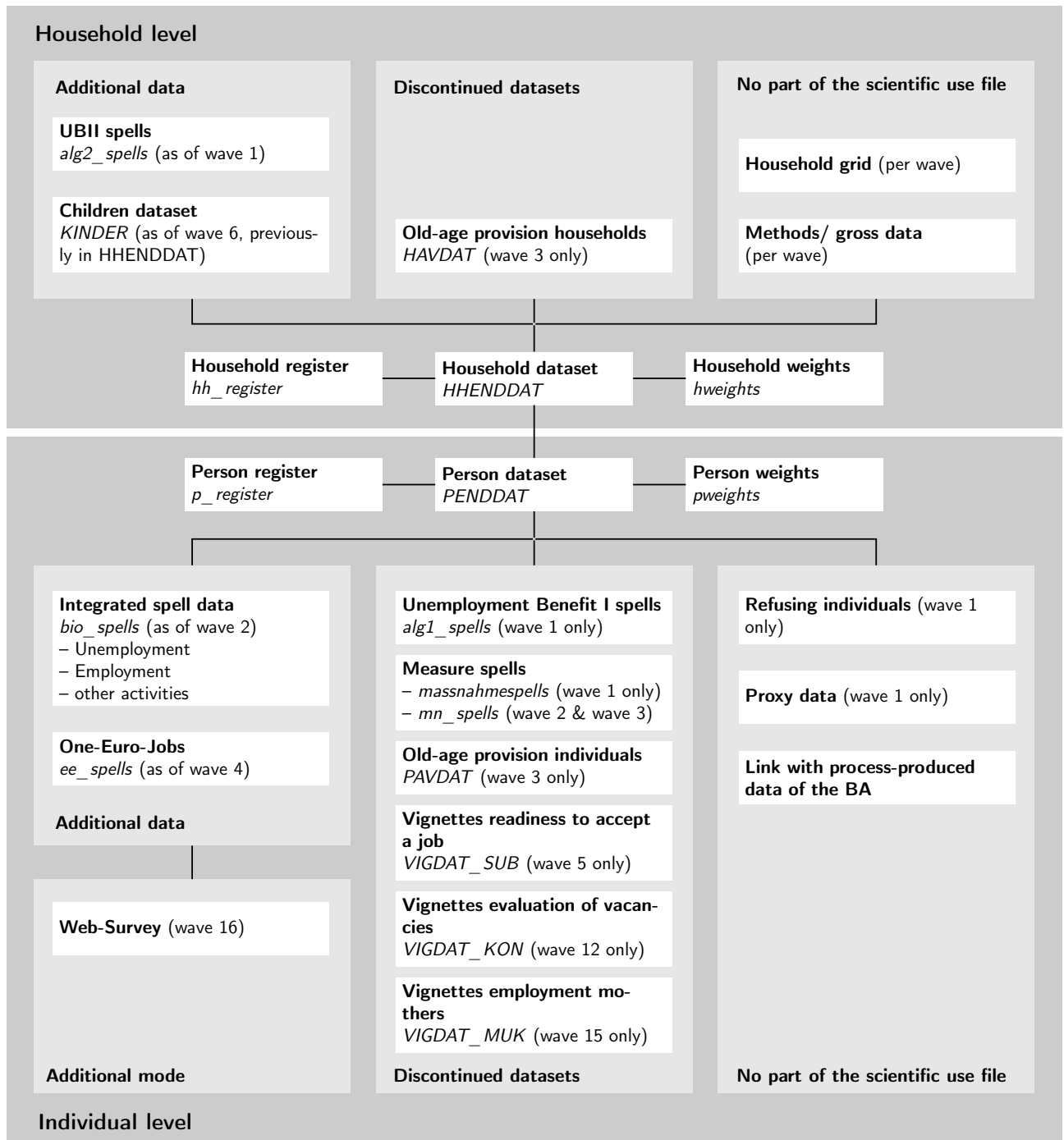
Figure 2: Dataset structure of PASS in wave 17
