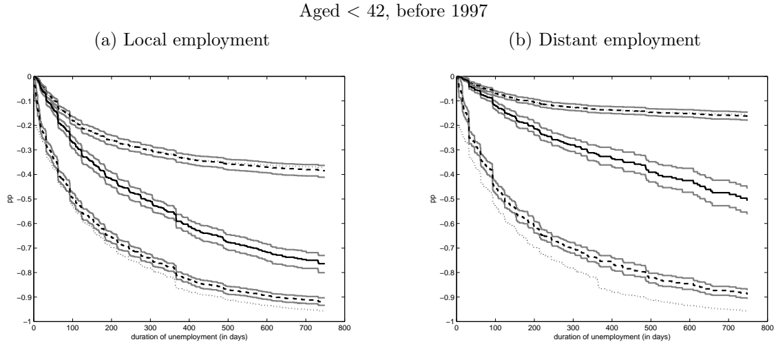
Figure 2: Estimated marginal survival functions with different dependence structures: KM Estimator (solid line); \tau = -0.8 (upper dashed line); \tau = 0.8 (lower dashed line); 95% and 5% bootstrap quantiles (grey dashed lines); Peterson bounds (dotted line)
