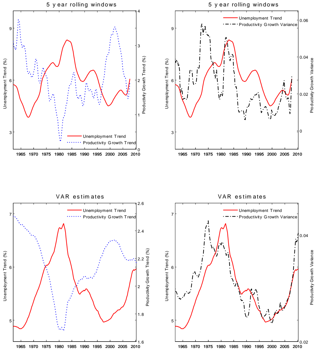
Figure 1: Long-run unemployment, long-run productivity growth and variance of productivity growth for the U.S., computed using five-year rolling windows for the charts on the first row and the time-varying VAR of section 3 for the charts on the second row.
