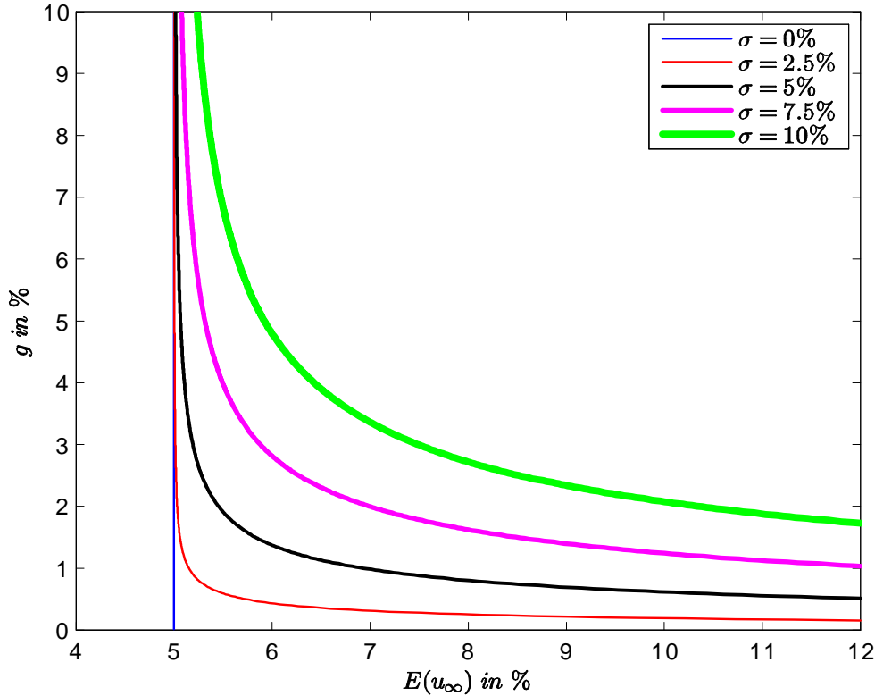
Figure 4: Model with downward real-wage rigidities: long-run relationships between the mean of unemployment, E(u_\infty) , and the mean of productivity growth, g , for different values of the standard deviation of productivity growth, \sigma . All variables in % at annual rates.
